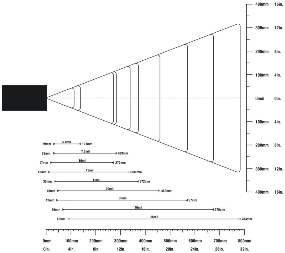
Figure 1-3 Long-range series
