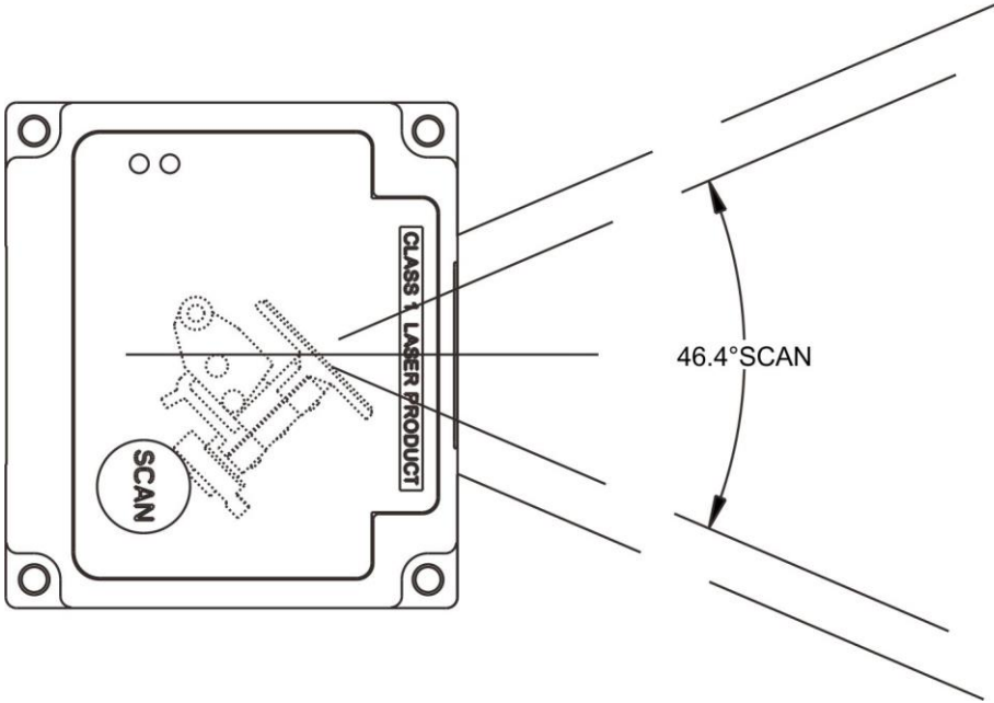
Figure 2-4 Scan angle
